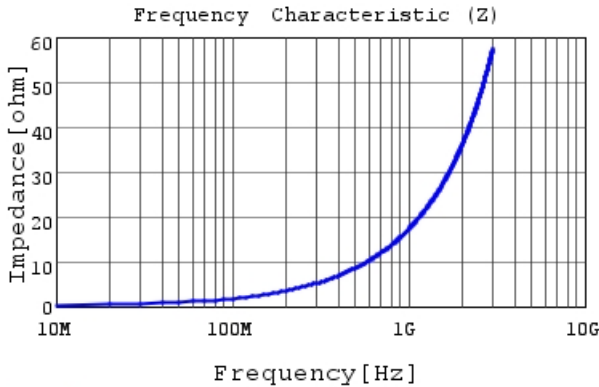
LQG15WH2N8S02 |Z|
