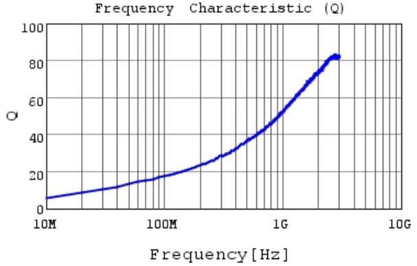
LQG15WH2N8S02 Q
