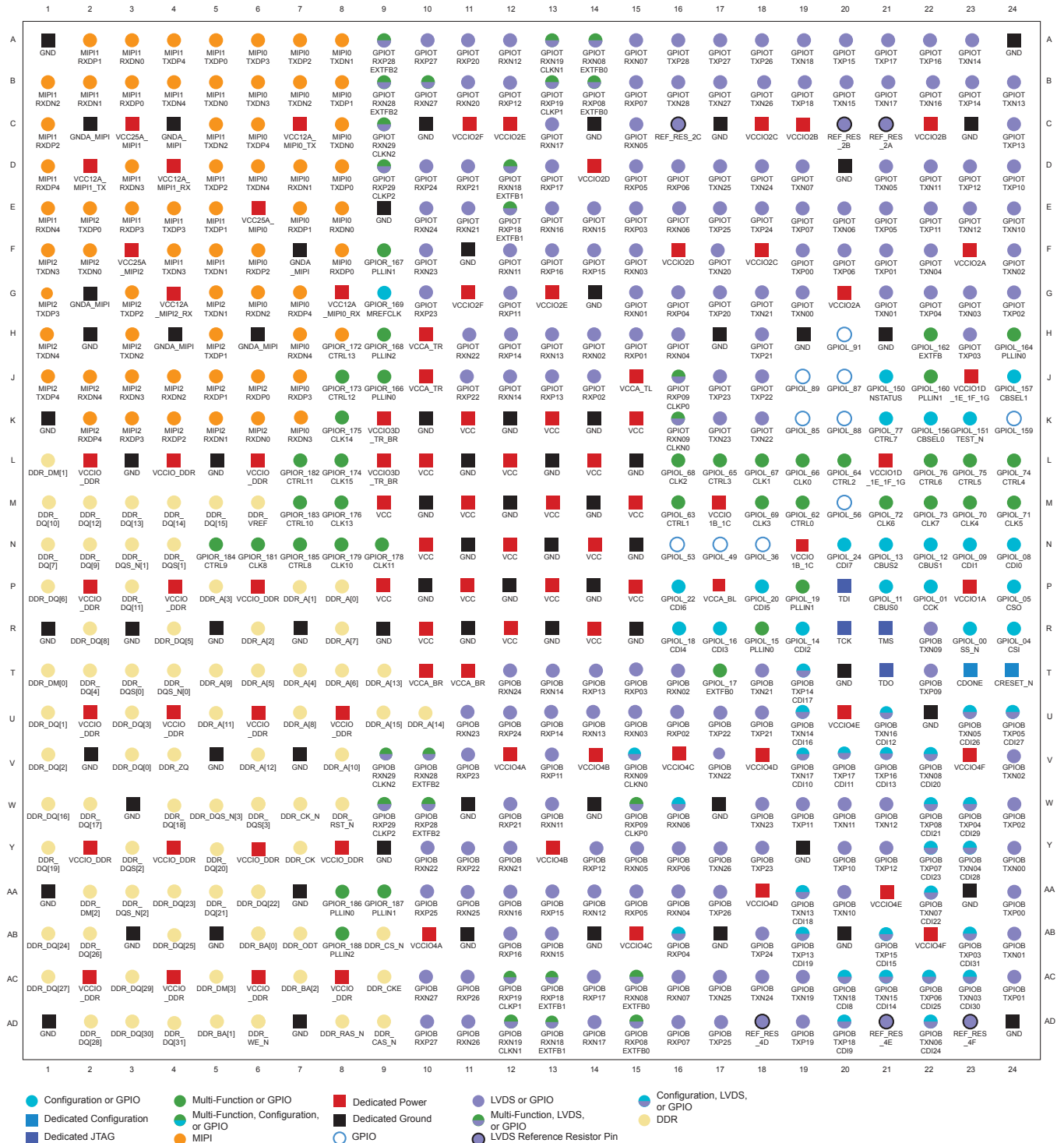
Figure 39: 576-Ball FBGA Pinout Diagram
