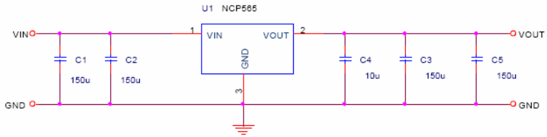
Figure 1: Schematic for NCP565 Fixed Demonstration Board
