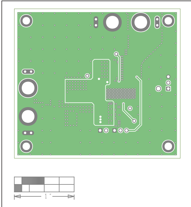
MAXM17537 EV Kit—Layer 3
