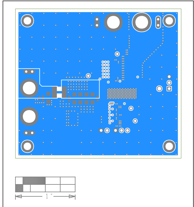
MAXM17537 EV Kit—Bottom Layer
