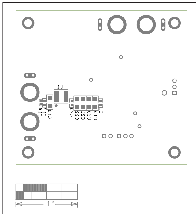
MAXM17537 EV Kit—Bottom Silkscreen
