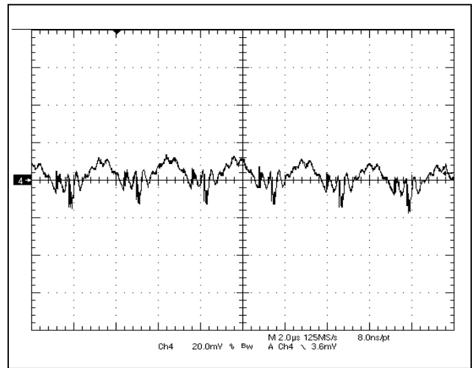
Fig-2.0V-5: Output voltage ripple (20mV/div.) for V_{out}=2.0V at full rated load current into a resistive load with external capacitance 47\mu F \times 2 ceramic + 1uF ceramic at V_{in}=12V . Time scale: 2 us/div.
