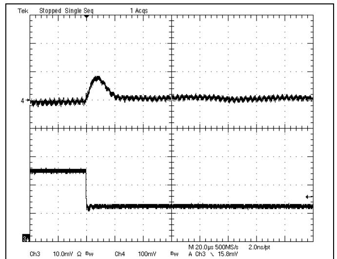
Fig-2.0V-7: Output voltage response for V_{out}=2.0V to negative load current step change from 5A to 2.5A with slew rate of -5A/us at V_{in}=12V . C_o=47\mu F \times 2 ceramic. Top trace: output voltage (100mV/div.) Bottom trace: load current (2A/div.) Time scale: 20us/div.
