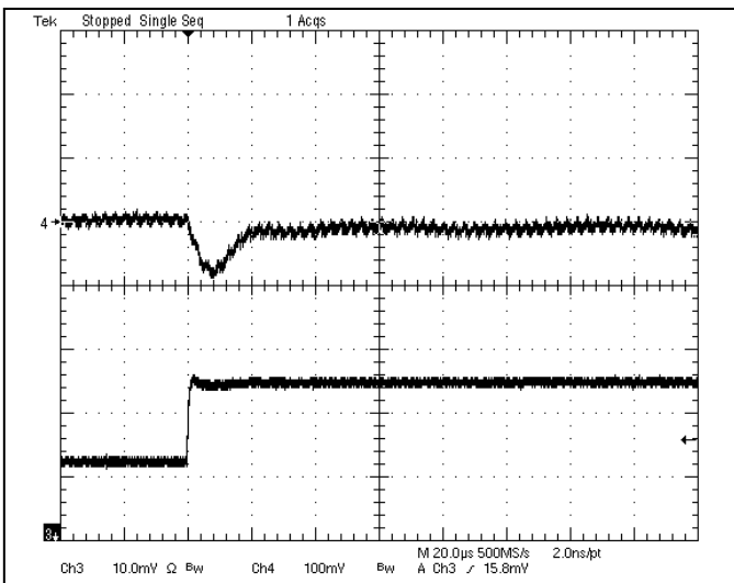
Fig-2.0V-6: Output voltage response for V_{out}=2.0V to positive load current step change from 2.5A to 5A with slew rate of 5A/us at V_{in}=12V . C_o=47\mu F \times 2 ceramic. Top trace: output voltage (100mV/div.) Bottom trace: load current (2A/div.) Time scale: 20us/div.
