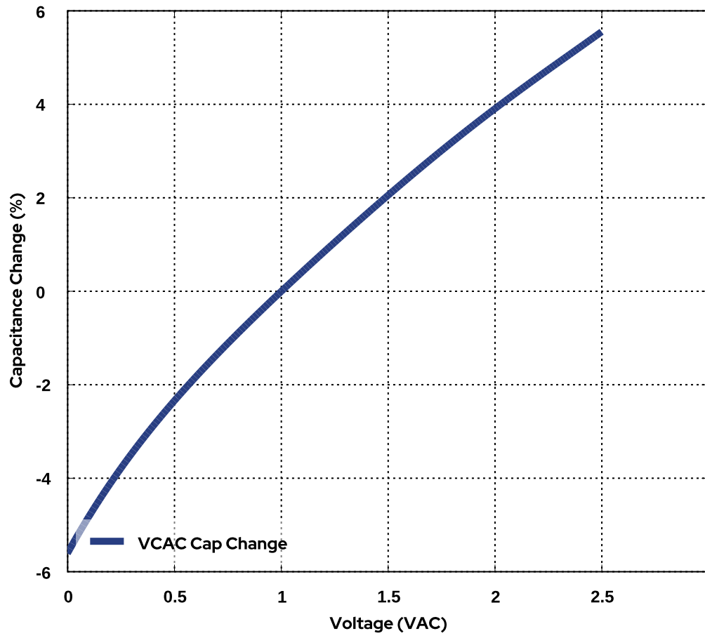
Capacitance Change versus AC Voltage
