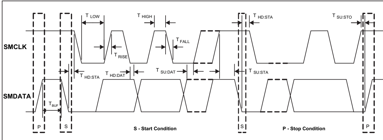
FIGURE 1-1: SMBus Timing.
