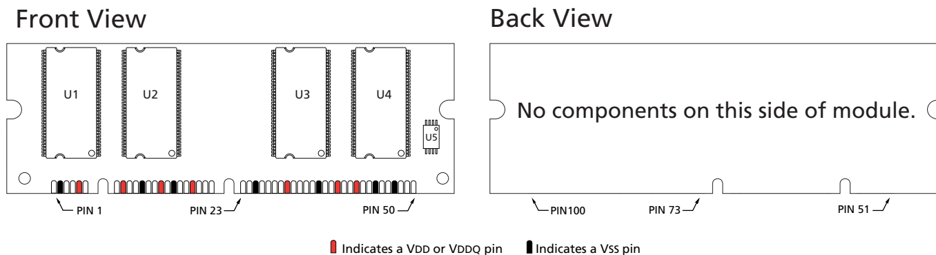
Figure 2: Module Layout
