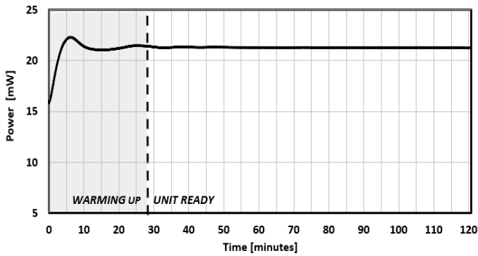
FIG. 9: WARM-UP TIME
