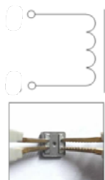
Figure 1. DCR test
