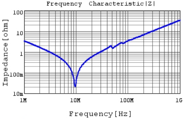
RCE7U2J473J5B1H03B |Z| DC0V, 25degC
