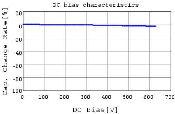
RCE7U2J473J5B1H03B C-DC bias capchange, 25.0
