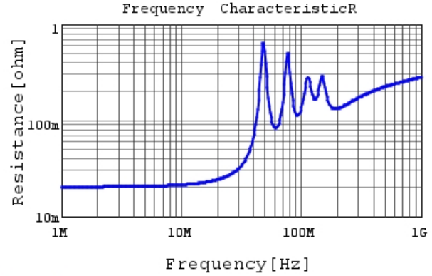
RCE7U2J473J5B1H03B R DC0V, 25degC
