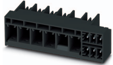
Figure shows a 5+6-pos. version with locking flange at position 5
