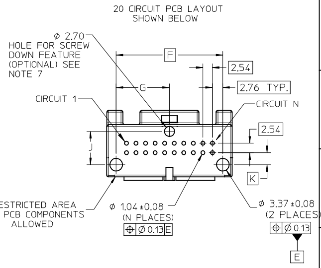
PCB LAYOUT: COMPONENT SIDE RECOMMENDED PCB THICKNESS: 1.57±0.17
