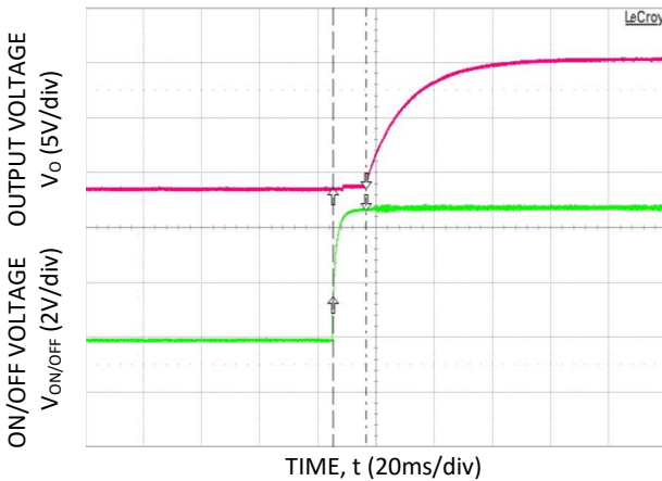
Figure 3. Start-up Using Remote On/Off (Vin: -48V DC , load independent)
