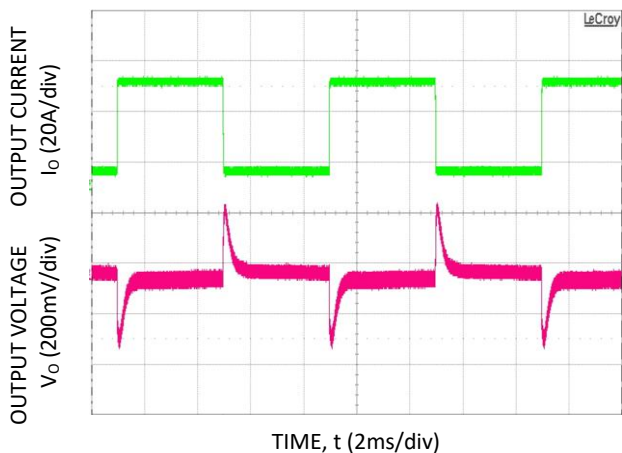
Figure 7. 12V transient response for 10 to 60% step load, Vin: -48V DC , slew rate 1A/μs.
