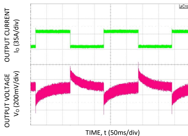
Figure 8. 12V transient response for 50 to 100% step load, Vin: -48V DC , slew rate 1A/μs.
