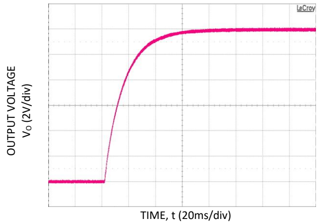
Figure 4. 12V start-up with 16,000µf external capacitance (Vin: -48V DC , full load)
