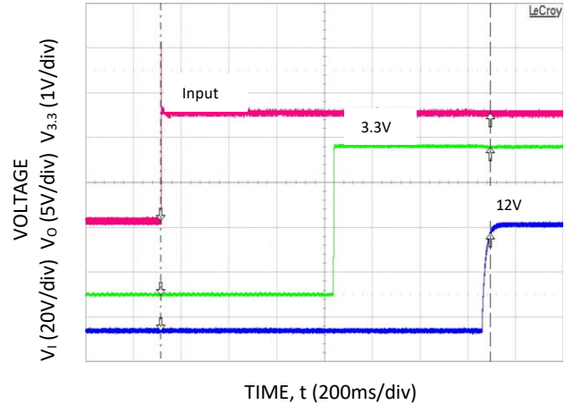
Figure 2. Input start up (Vin: -48V DC , full load).
