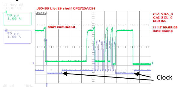
Figure 14. Example waveforms showing clock stretch
