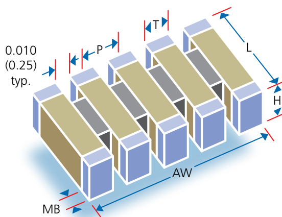
Dimensions - inches/mm
