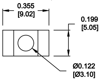
SADDLE WASHER
